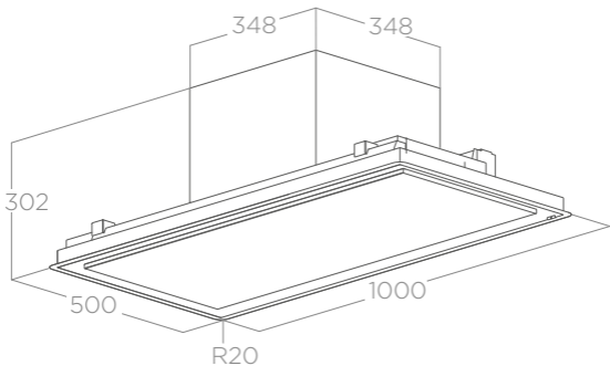
FALSE CEILING CUT: 480X980
