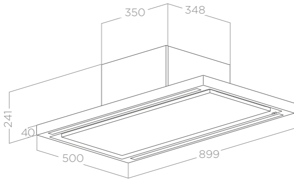
FALSE CEILING CUT: 480X880
